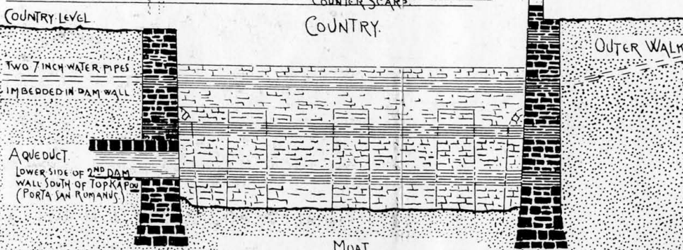
SHOWING THE BUTTRESSING TO DAM WALLS
